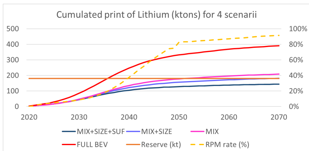
Figure 5 Evolution of the cumulated lithium material print for 4 mobility scenarios: FULL BEV = all electric without sufficiency. MIX = Mix electric and hybrid gaz. MIX+SIZE = MIX + optimization of vehicle size. MIX+SIZE+SUF = MIX+SIZE+sufficiency (reduction of private car use and increased carpooling).
